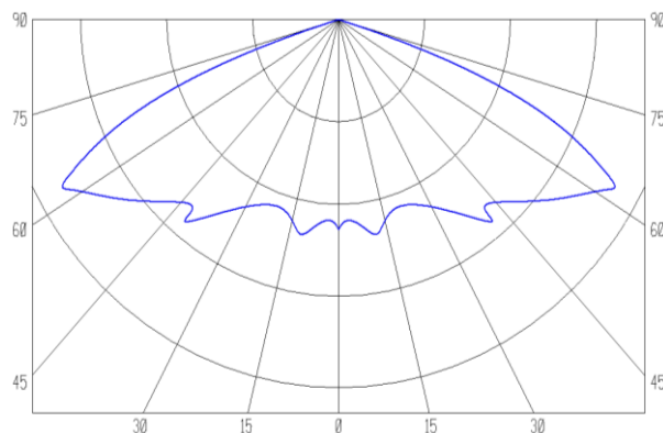
Figure 1: Indicative acceptable illumination pattern
